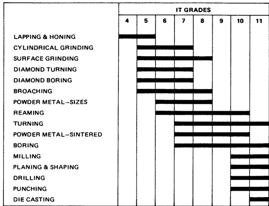
FIG. 6-6 MACHINING PROCESSES (ANSI B4.2)
